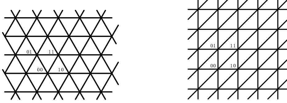
Figure 2: Triangular Lattice
