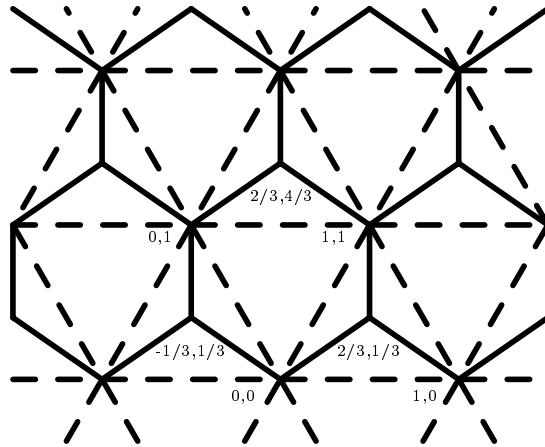
Figure 4: Hexagonal Lattice
