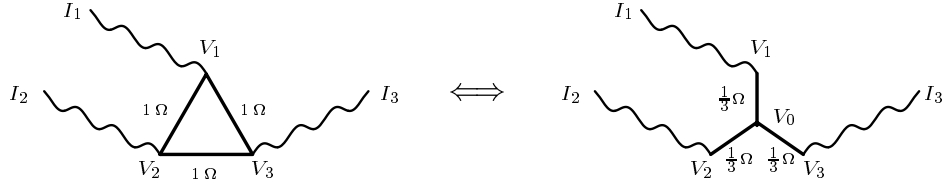
Figure 3: \Delta -Y Transformation
